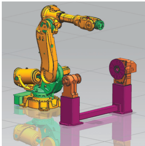
Six- and seven-axis robotic configurations can be defined and used in NX, including robots on rails and work positioners.
