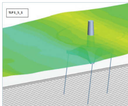
The waves-induced movement of anchored objects.
